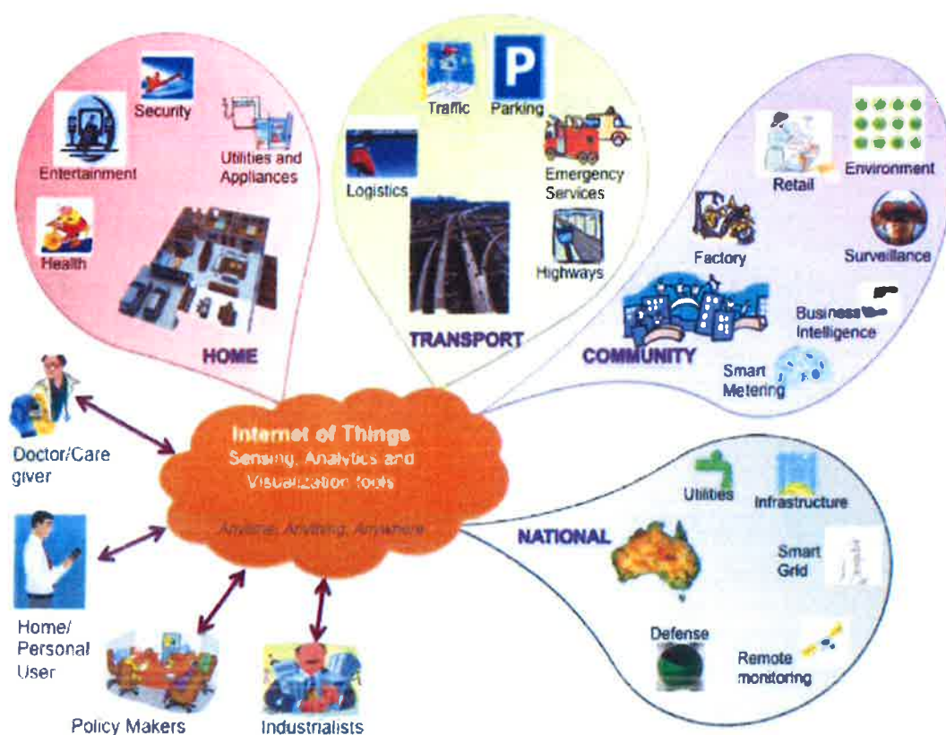
Figure 2 - IoT applications
